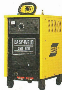
EasyWeld SSR 600
